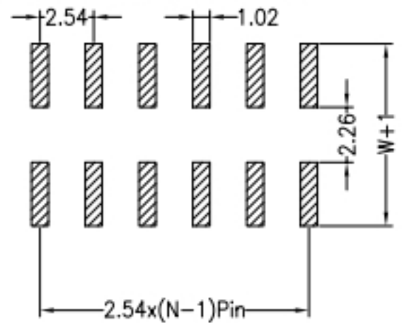
Recommended P.C.B Layout(Top Side) (PCB BOARD TOLERANCE±0.05)
