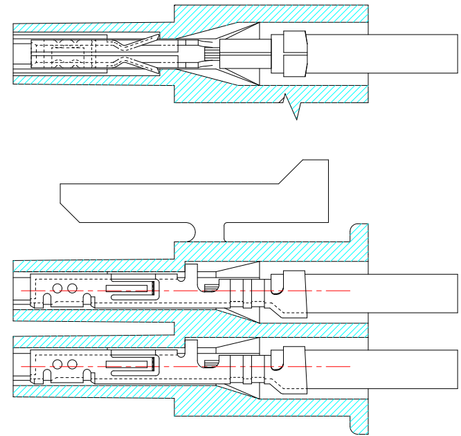
SECTIONAL DRAWING
